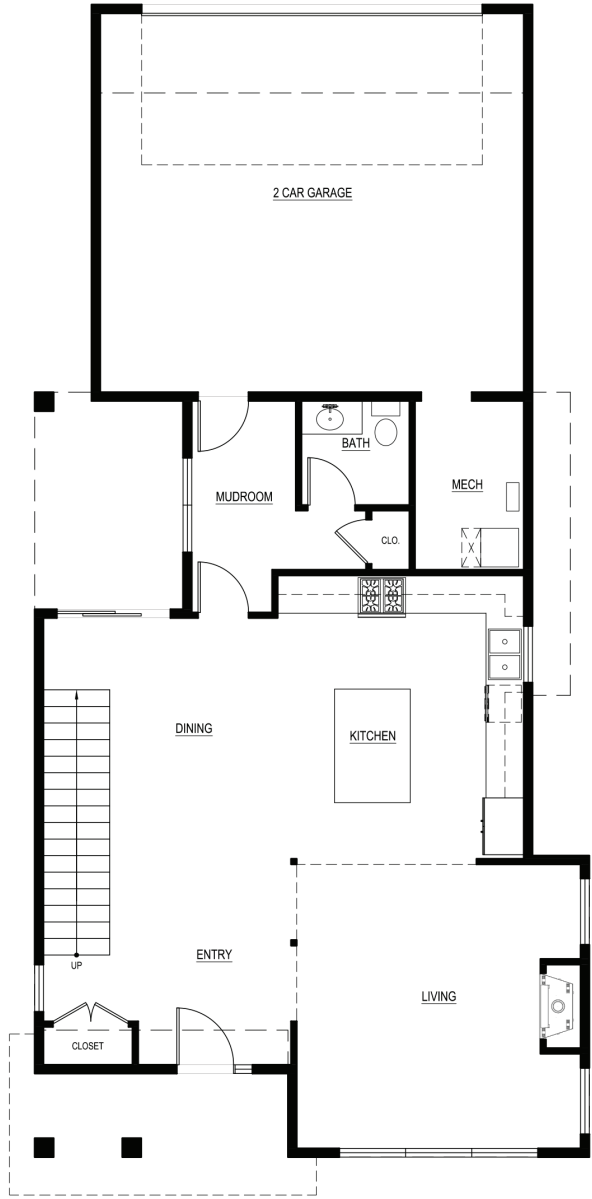
MAIN FLOOR
